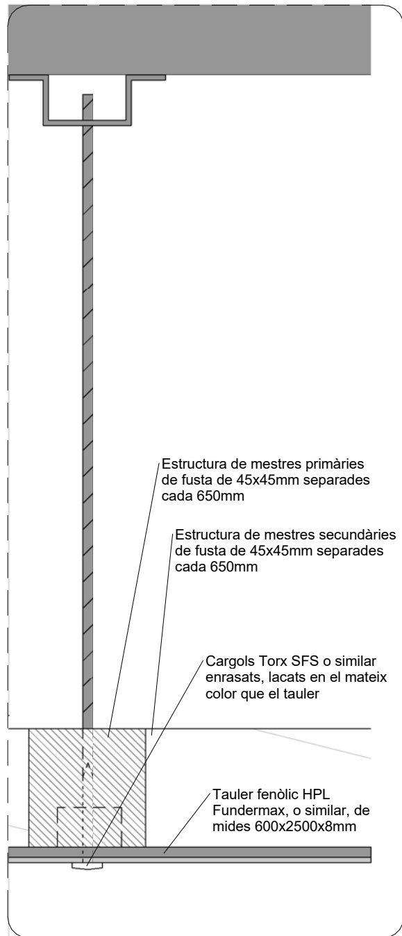
B3-DET4 (e 1 : 2)
