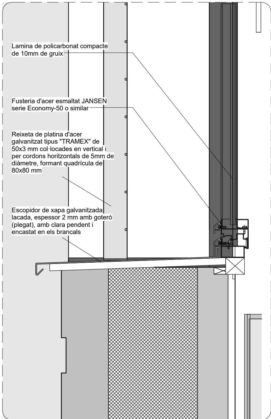
B3-DET1 (e 1 : 5)
