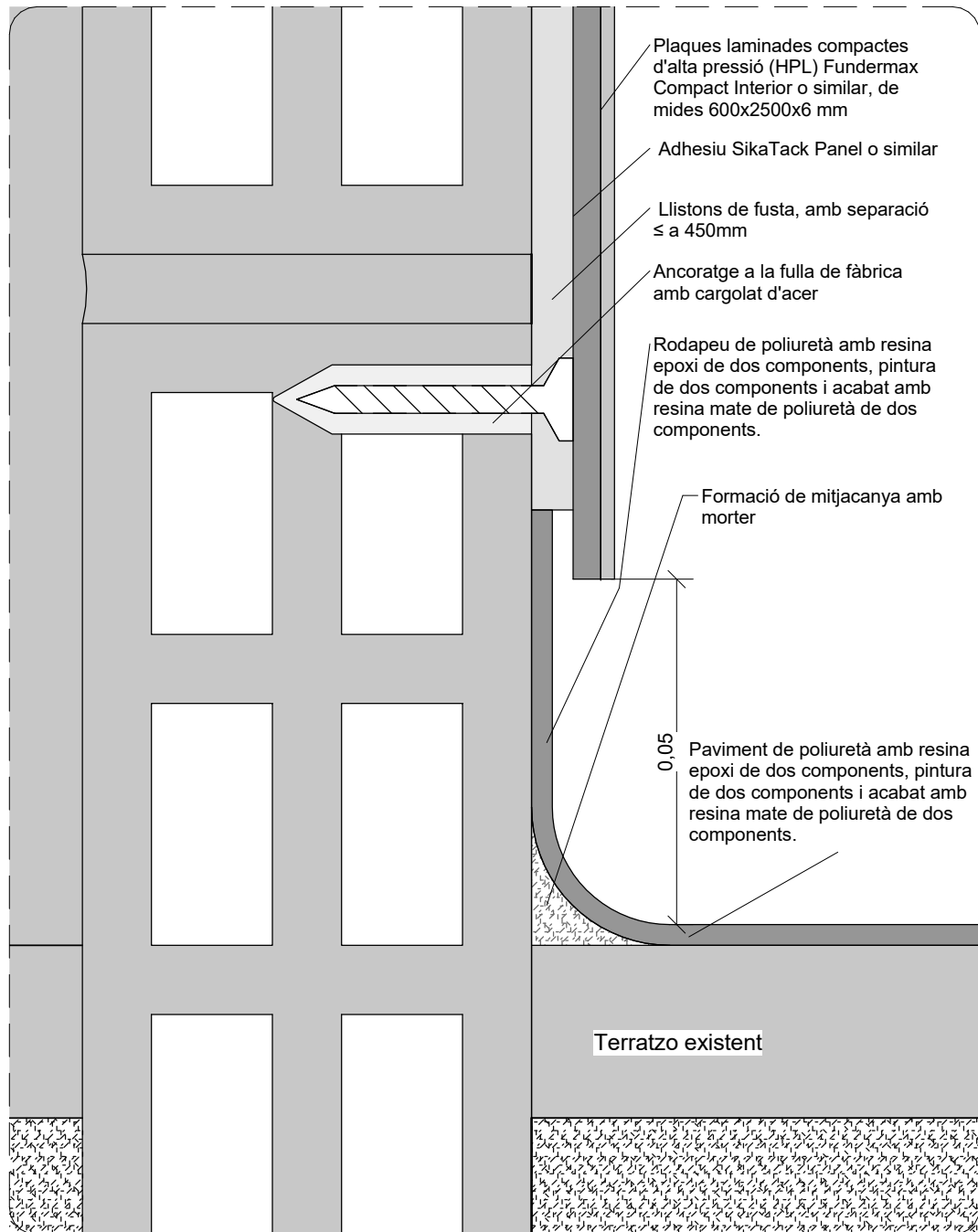
B3-DET2 (e 1 : 1)
